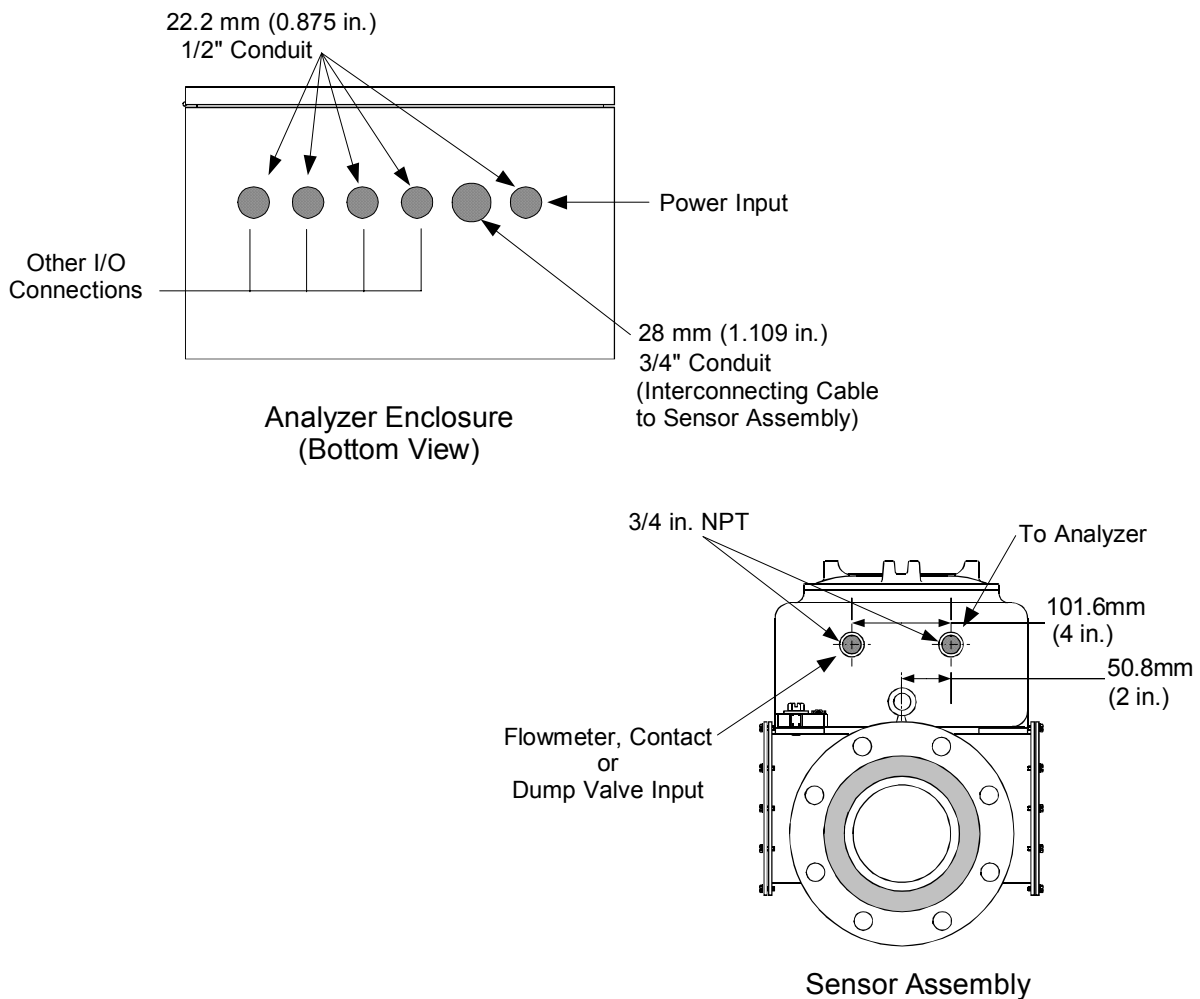
Figure 1 Conduit Connections
