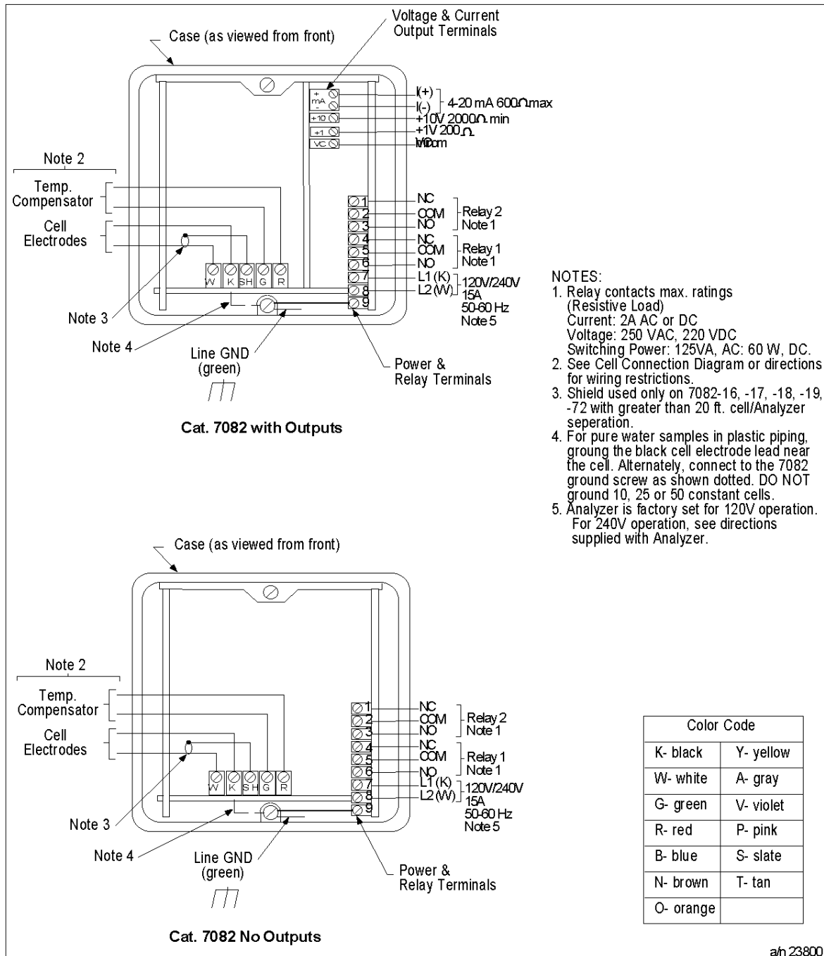
Figure 0-1 Terminal Connections
